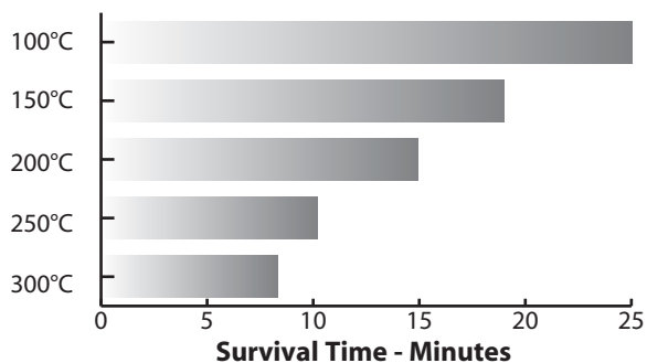
Thermal Protection Duration
